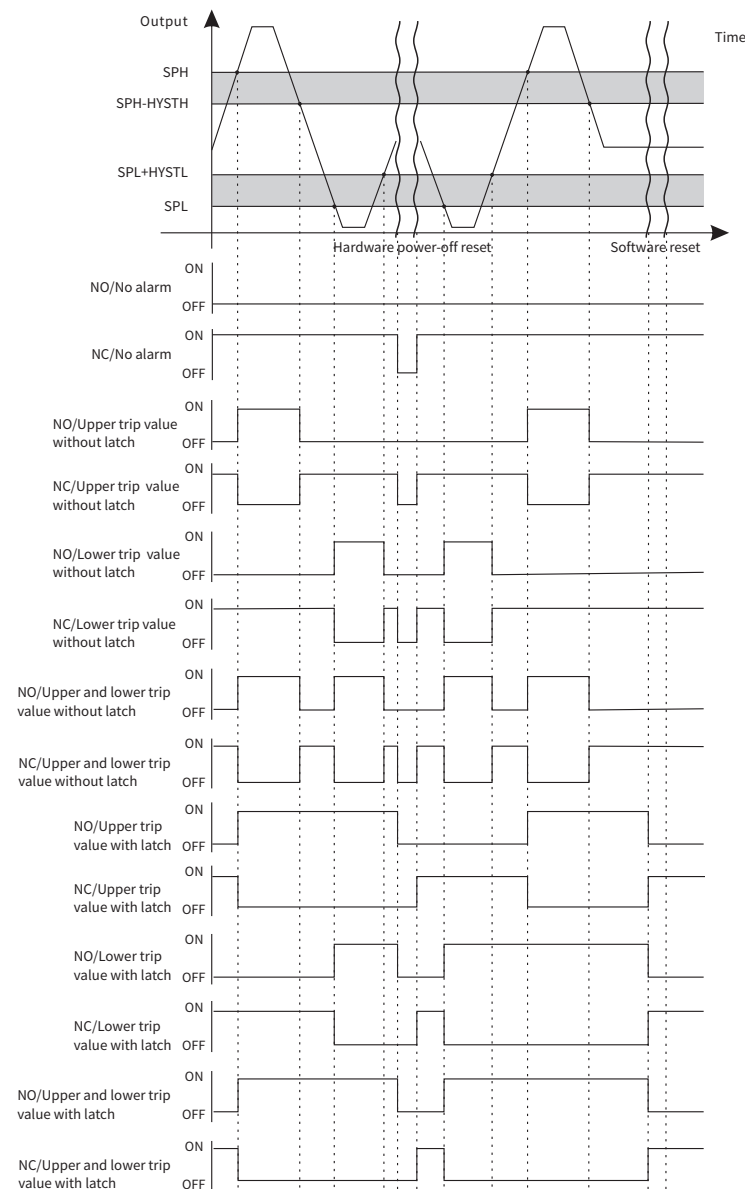
Relationship between relay alarm mode and measured value
